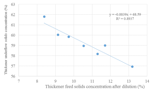
Figure 4. The effect of solids concentration during flocculation on the thickener performance
